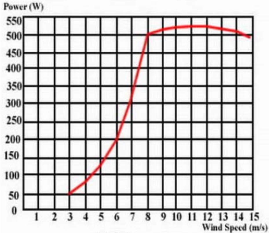
500W power curve
