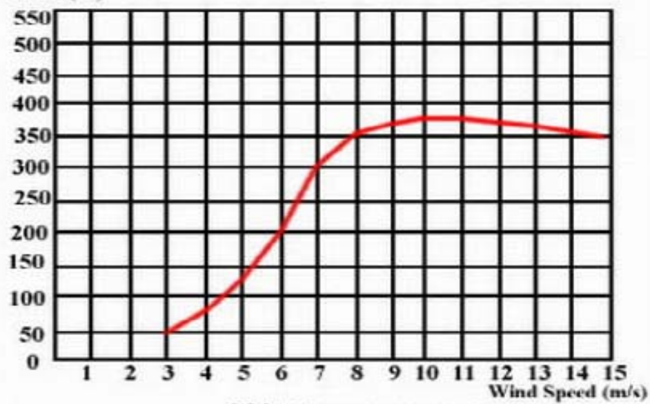
300W power curve
