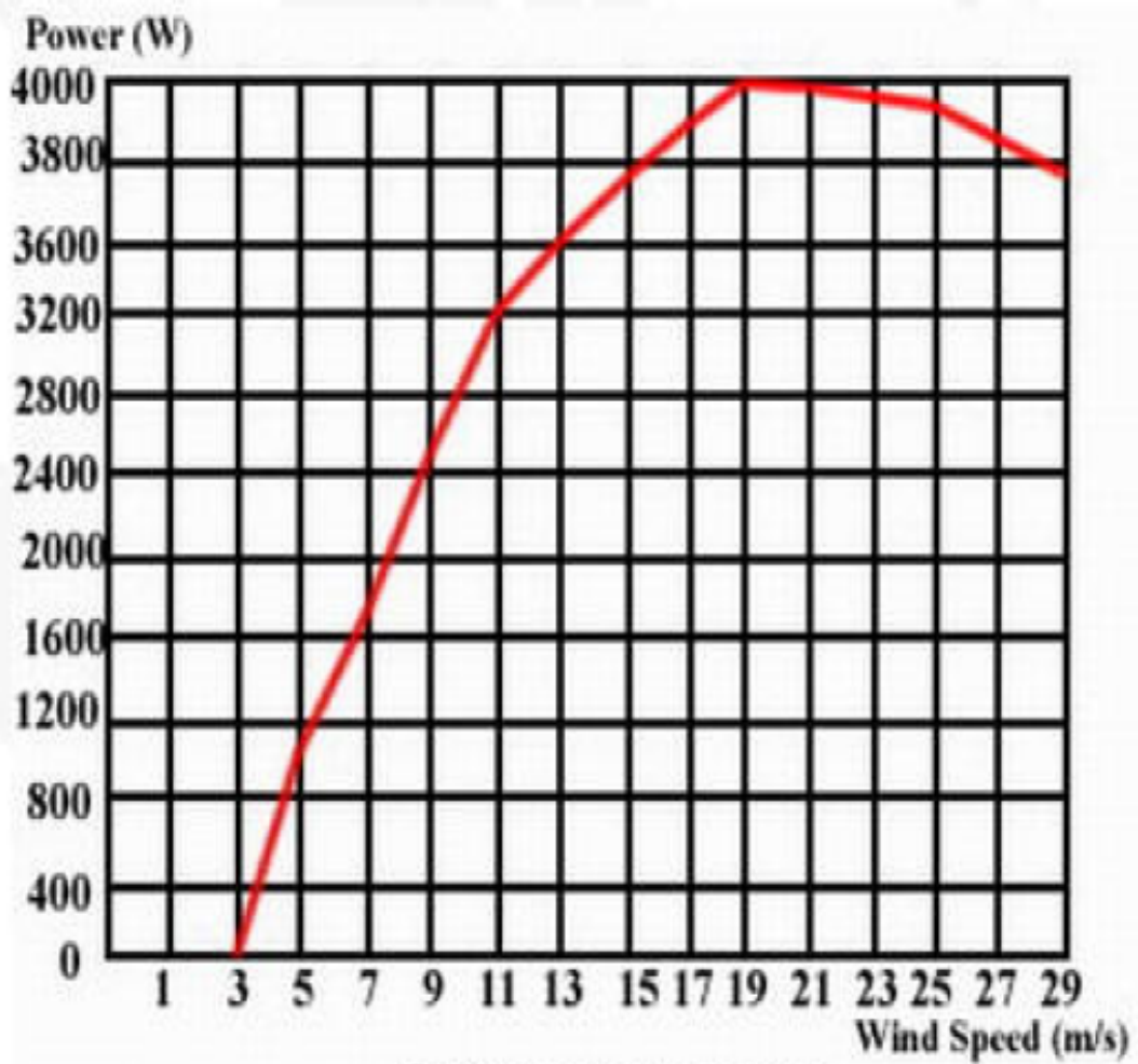
3KW power curve
