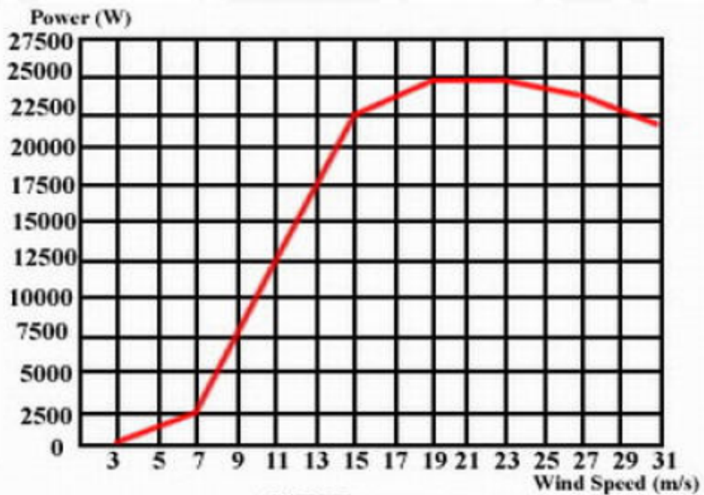
20KW power curve
