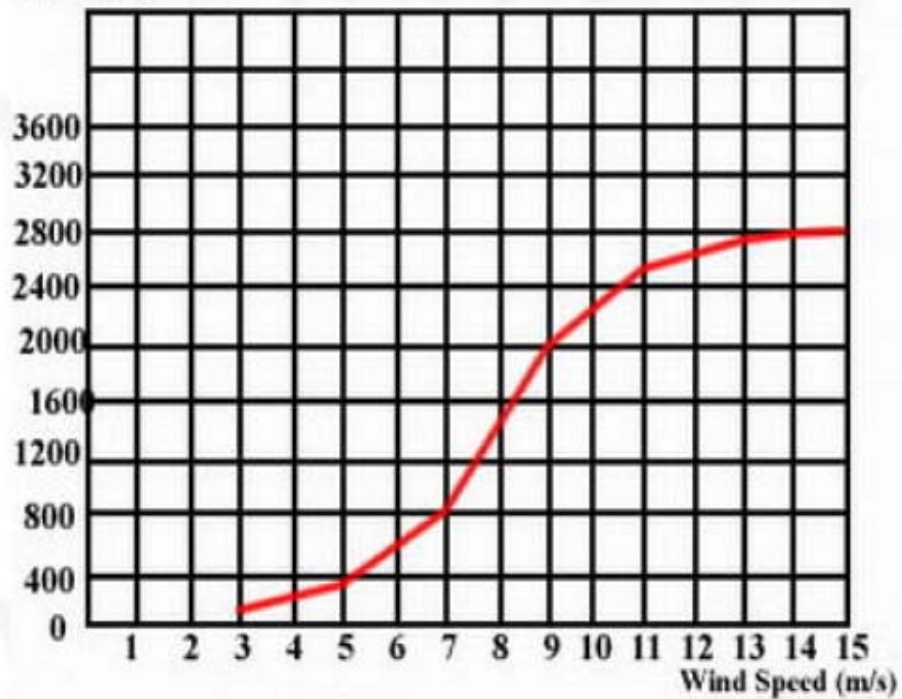
2KW power curve
